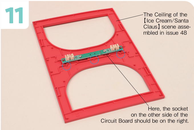
Get ready the Ceiling of the 【Ice Cream/Santa Claus】 scene assembled in issue 48 and identify the protrusions circled in blue. Align the LEDs with these protrusions and affix the Cable with LEDs.
