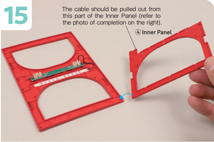
Remove the Battery Box and assemble the ④ Inner Panel to the Ceiling Top Panel.
