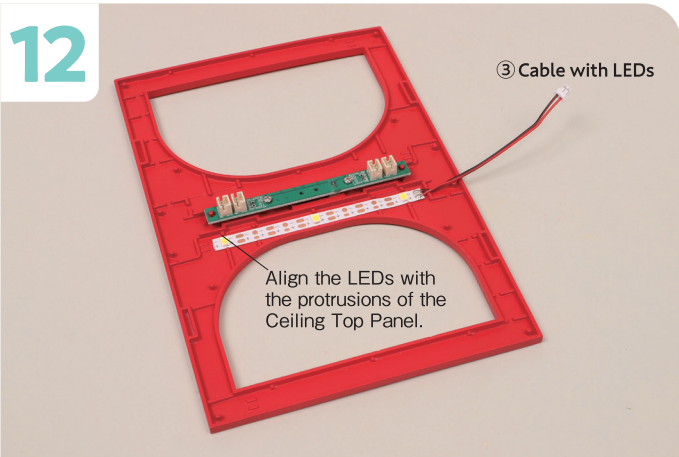
Affix the ③ Cable with LEDs in line with the indentation in the Ceiling Top Panel, with the LEDs aligned with the protrusions identified in step 11.
