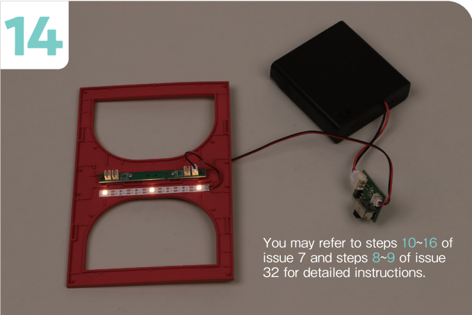
Insert the connector of the Connection Cable into the socket on the other side of the Ceiling, connect it to a Battery Box and check if the LEDs light up properly.
